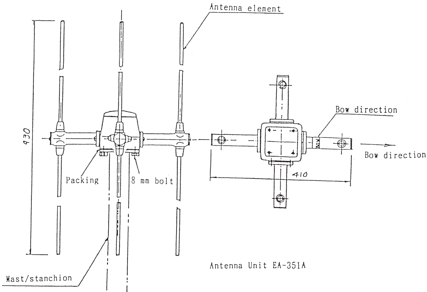
Diagram 3 Antenna Unit
